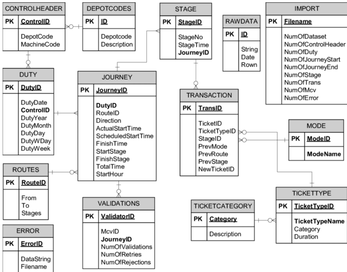
Figure A.1: Full-size Entity Relationship Diagram (ERD).
